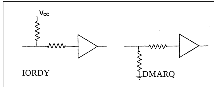
Figure 5.9 Ultra DMA termination with pull-up or pull-down
