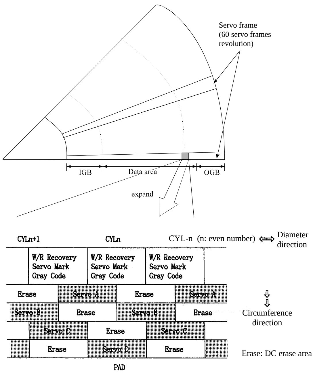
Figure 4.7 Physical sector servo configuration on disk surface
