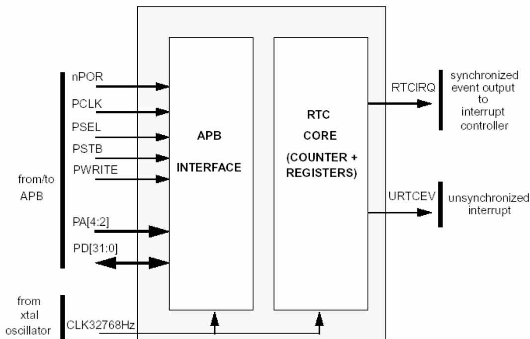
Figure 10-5 RTC Connection
