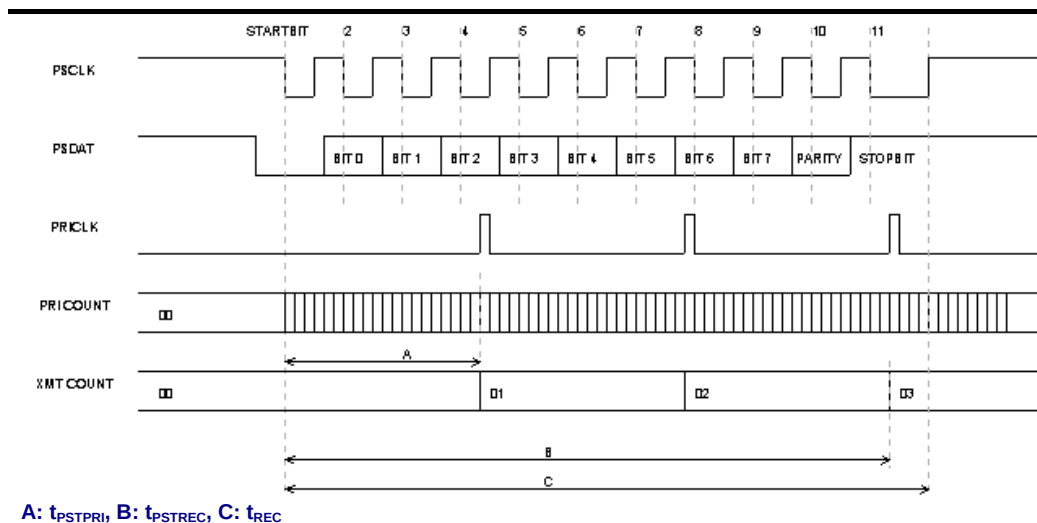
Figure 10-4 PS/2 Controller Receiving Data Timing Diagram
