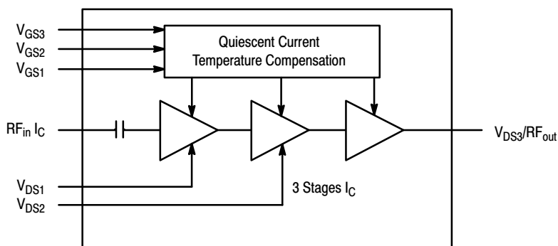
Figure 1. Block Diagram
