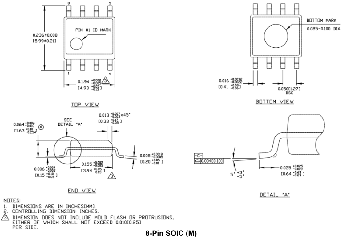
8-Pin SOIC (M)
