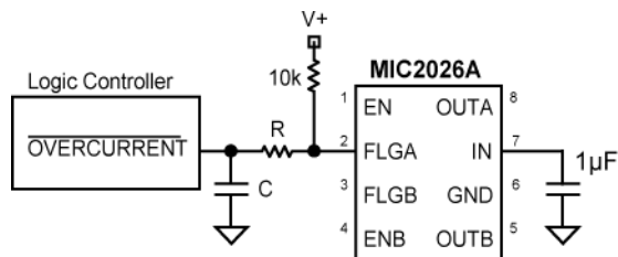
Figure 4. Transient Filter
