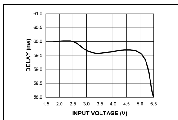
FIGURE 2-6: MIC2090 Auto-Reset Time vs. Input Voltage.
