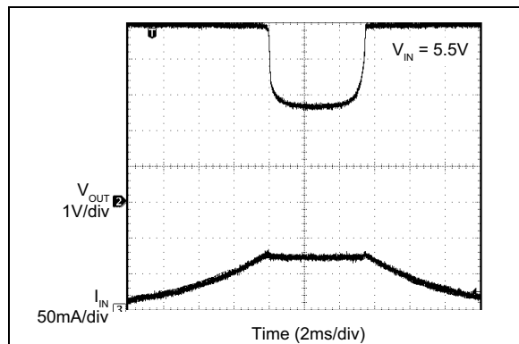
FIGURE 2-45: I_{OUT} Current Limiting for V_{OUT} > 1.8V (-1 Version).
