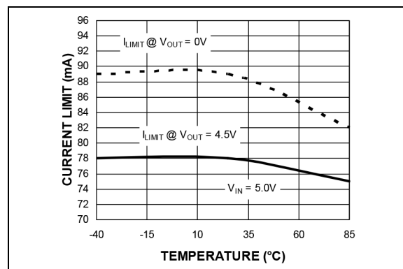
FIGURE 2-18: MIC2090 Current-Limit vs. Temperature.
