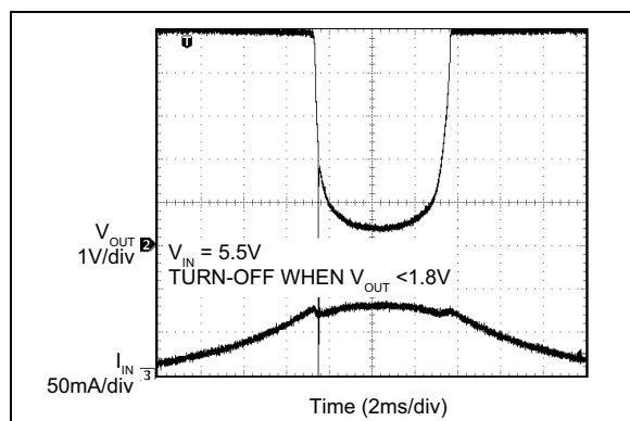
FIGURE 2-44: I_{OUT} Current Limiting for V_{OUT} < 1.8V (-1 Version).
