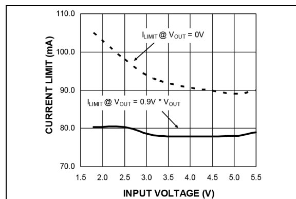
FIGURE 2-4: MIC2090 Current-Limit vs. Input Voltage.
