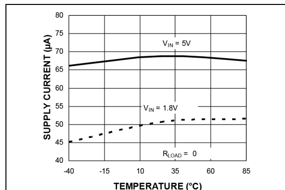
FIGURE 2-16: V_{IN} Supply Current vs. Temperature.
