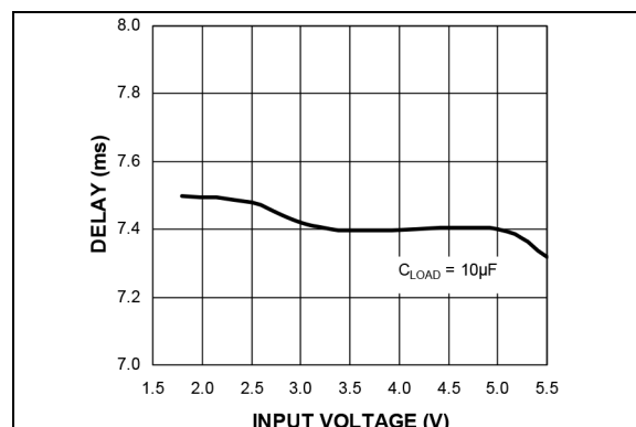
FIGURE 2-5: MIC2090 FAULT/ Delay vs. Input Voltage.
