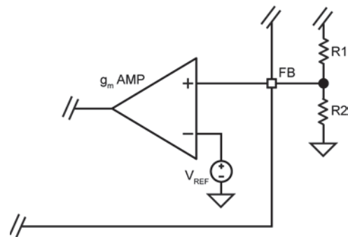
Figure 7. Voltage-Divider Configuration
