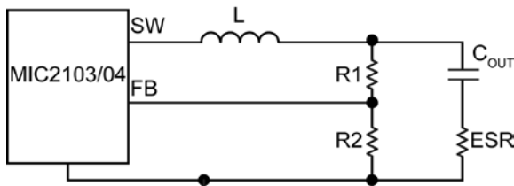
Figure 8a. Enough Ripple at FB
