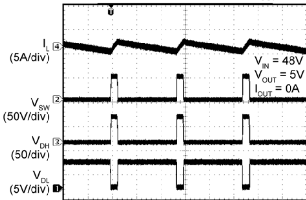
MIC2104 Switching Waveforms; I_{OUT} = 0A
