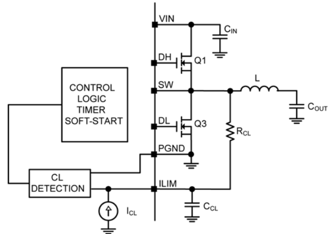
Figure 4. MIC2103/04 Current Limiting Circuit
