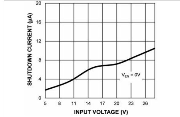
FIGURE 2-4: V_{IN} Shutdown Current vs. Input Voltage (MIC2125).
