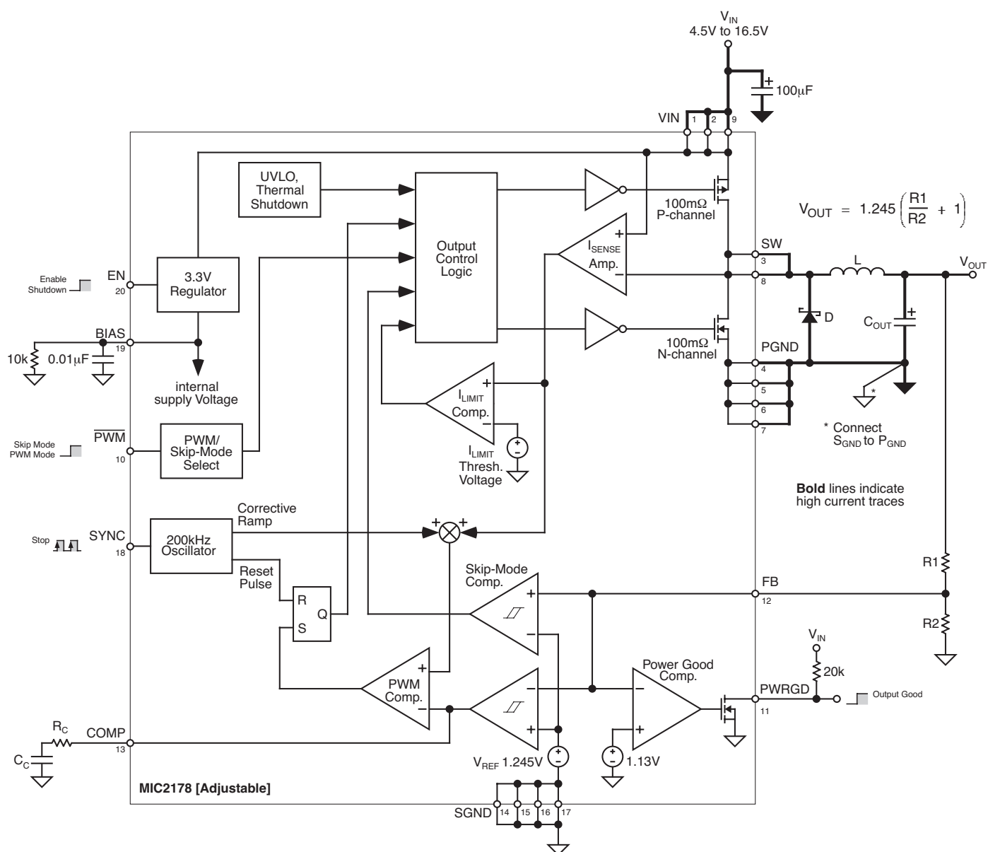
Block Diagram
