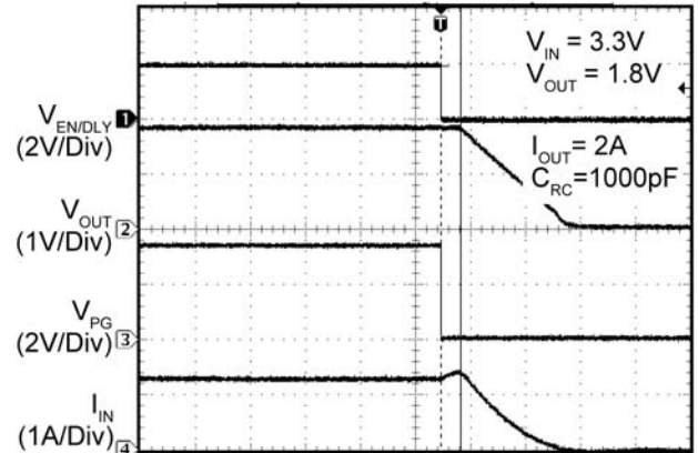
Enable Turn-Off
