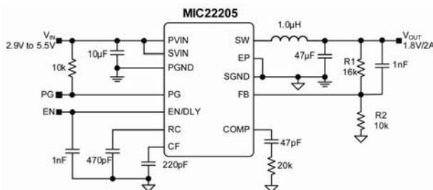
MIC22205 2A 1MHz Synchronous Output Converter
