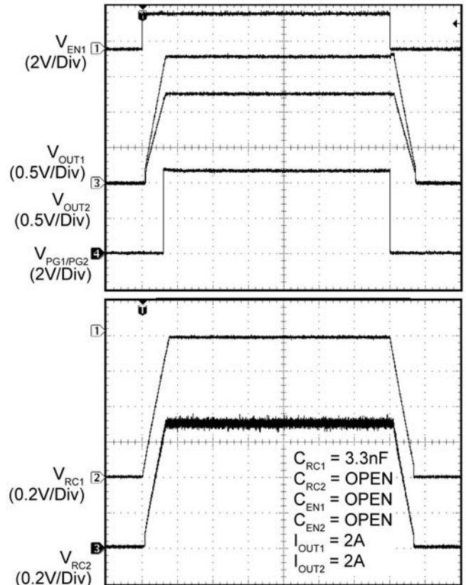
4.0ms/div
