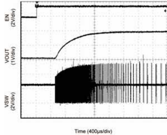
Start-Up Waveform
