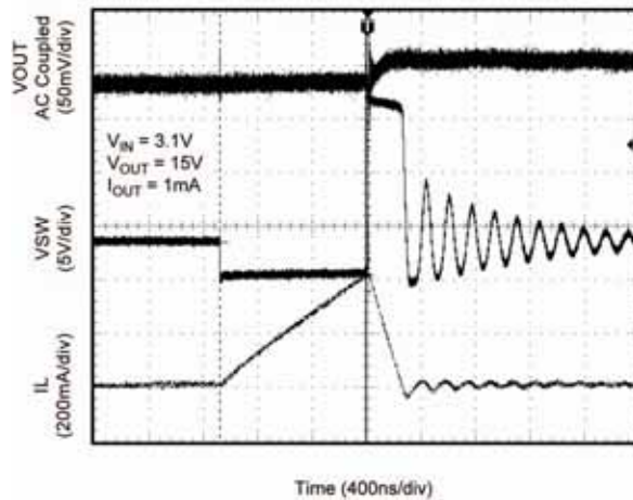
Switching Waveform
