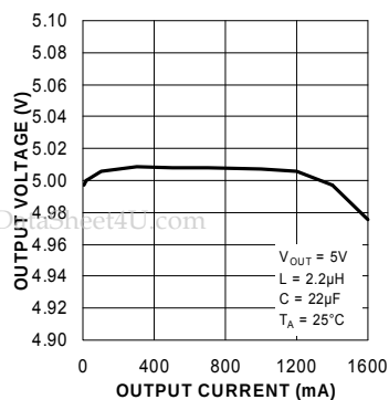
Load Regulation
