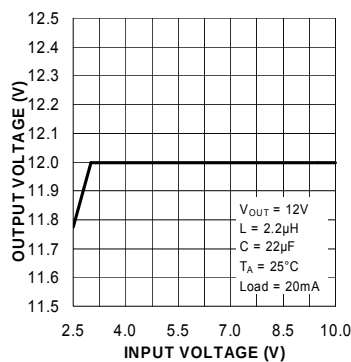
Line Regulation
