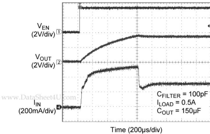
Startup Waveform
