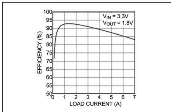
FIGURE 5-1: Efficiency Curve.
