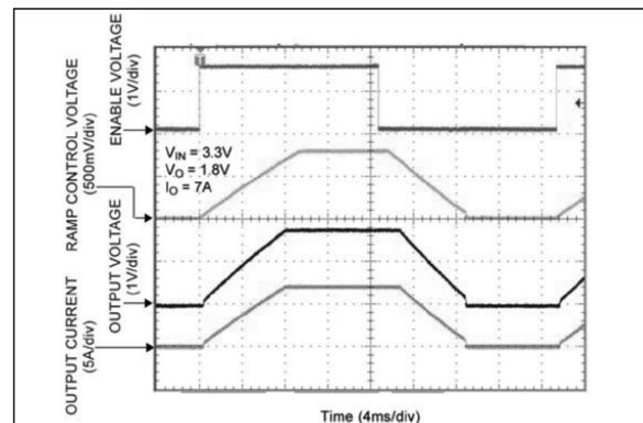
FIGURE 2-18: Start-Up/Shutdown ( C_{RC} = 10\text{ nF} ).
