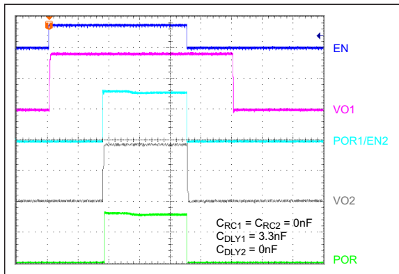
FIGURE 5-4: Window Sequencing Example.
