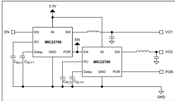
FIGURE 5-3: Sequencing MIC22700 Circuit.
