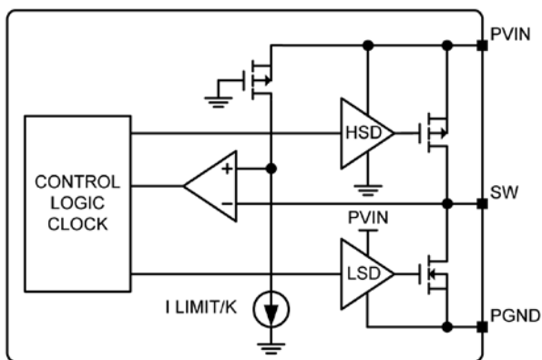
Figure 7. Current-Limit Detail
