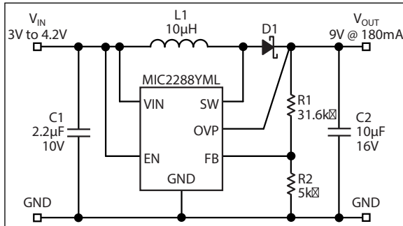
FIGURE 6-2: 3.0V to 4.2V V_{IN} to 9V _{OUT} @ 180 mA.
