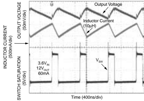
Switching Waveforms
