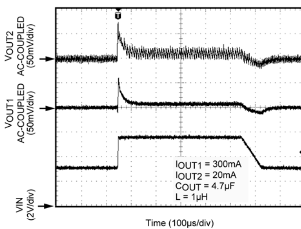
Line Transient
