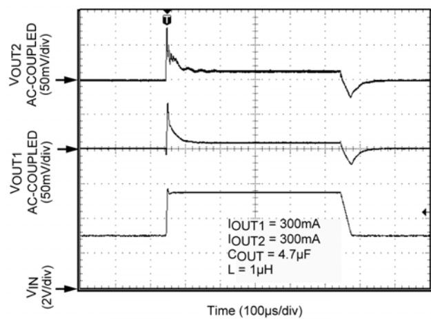
Line Transient
