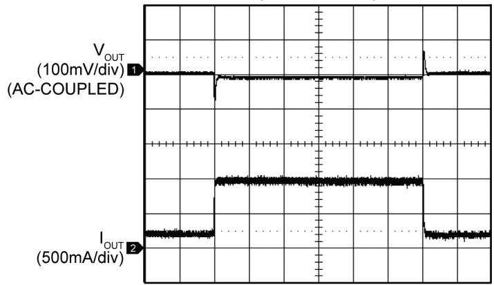
Load Transient (200mA to 1A)
