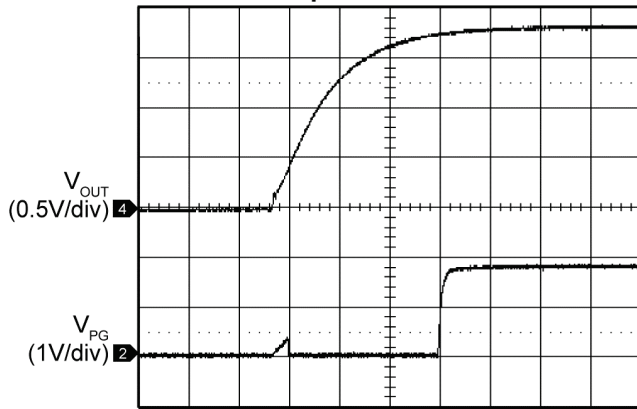
Start-Up and PG Waveform
