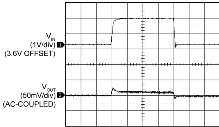
Line Transient (3.6V to 5.5V @1A Load)
