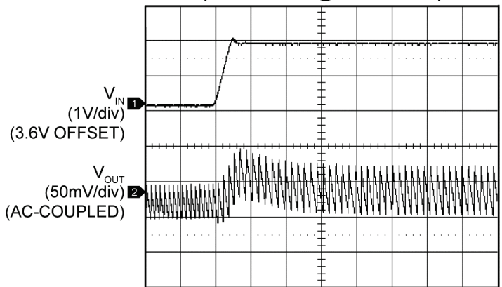
Line Transient (3.6V to 5.5V @ 20mA Load)
