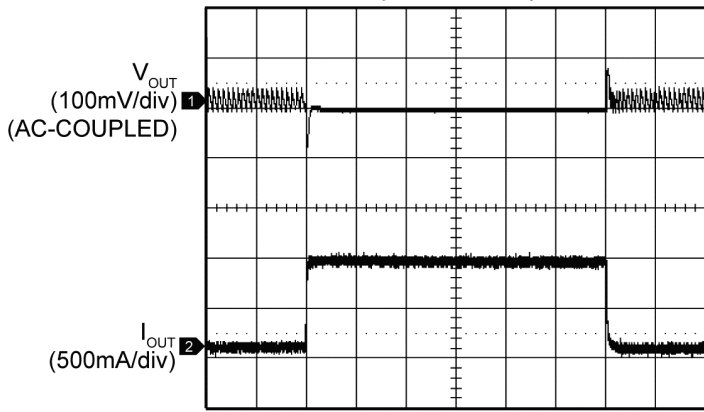
Load Transient (50mA to 1A)
