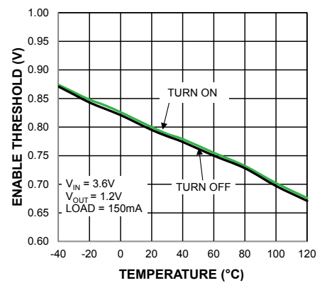
Enable Thresholds vs. Temperature
