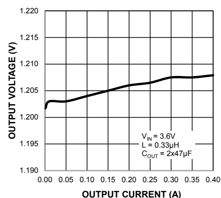
Output Voltage vs. Output Current (HLL)
