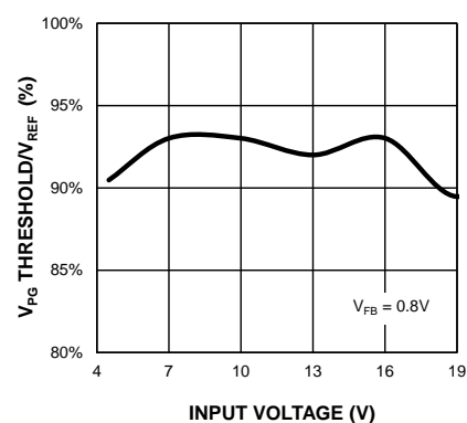
PG Threshold/VREF Ratio vs. Input Voltage
