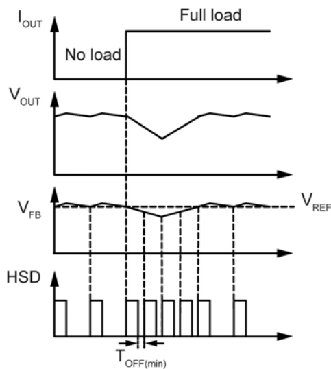
Figure 3. MIC26603-ZA Load Transient Response
