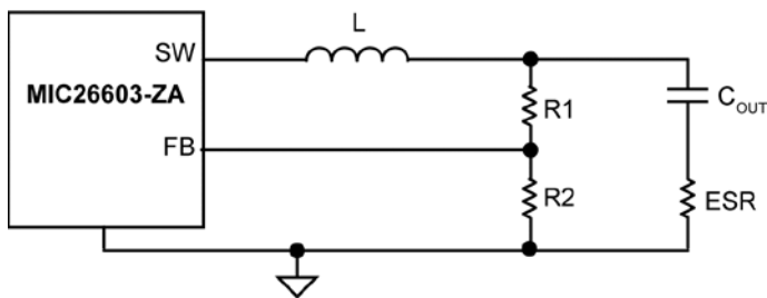
Figure 5. Enough Ripple at FB
