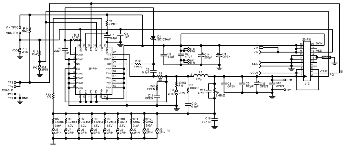
Figure 10. Schematic of MIC26603-ZA Evaluation Board (J11, R13, R15 are for testing purposes)
