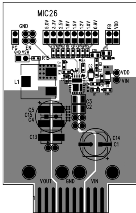
MIC26603-ZA Evaluation Board Top Layer
