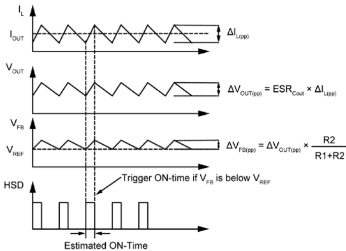
Figure 2. MIC26603-ZA Control Loop Timing
