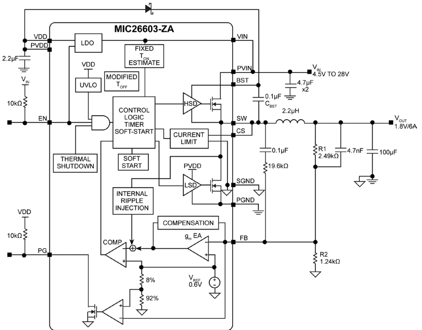
Figure 1. MIC26603-ZA Block Diagram
