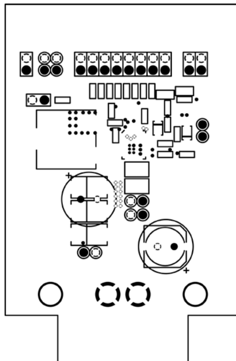
MIC26603-ZA Evaluation Board Mid-Layer 1 (Ground Plane)
