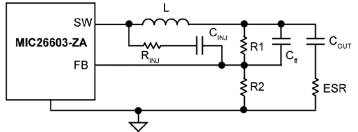
Figure 7. Invisible Ripple at FB
