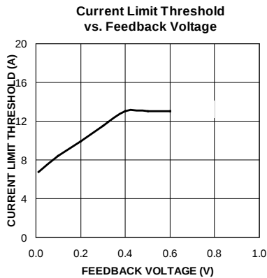
Figure 4. MIC26603-ZA Current-Limit Foldback Characteristic
