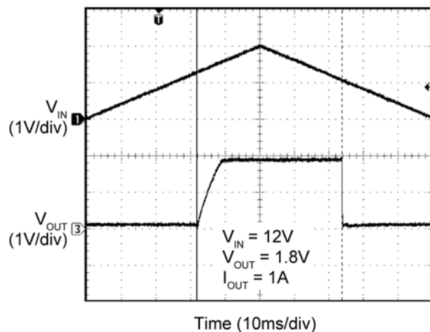
Enable Thesholds
