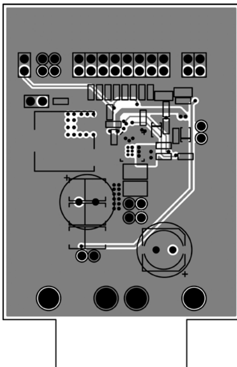
MIC26603-ZA Evaluation Board Mid-Layer 2
