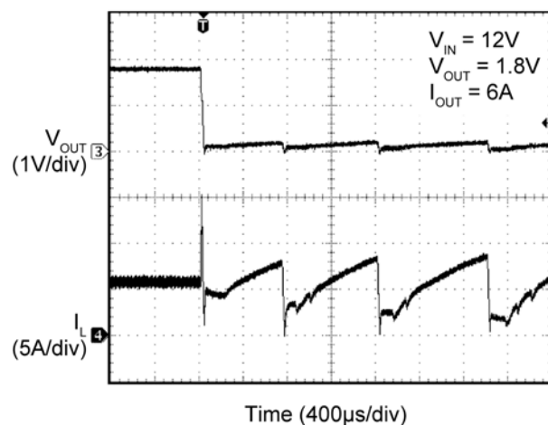
Short Circuit
