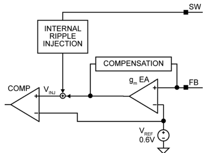
Figure 9. Internal Ripple Injection
