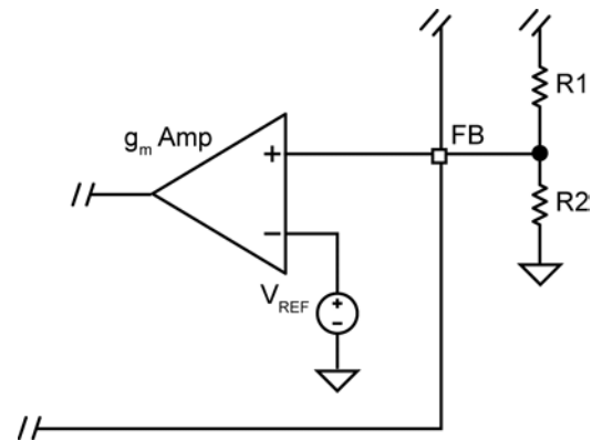
Figure 8. Voltage-Divider Configuration
