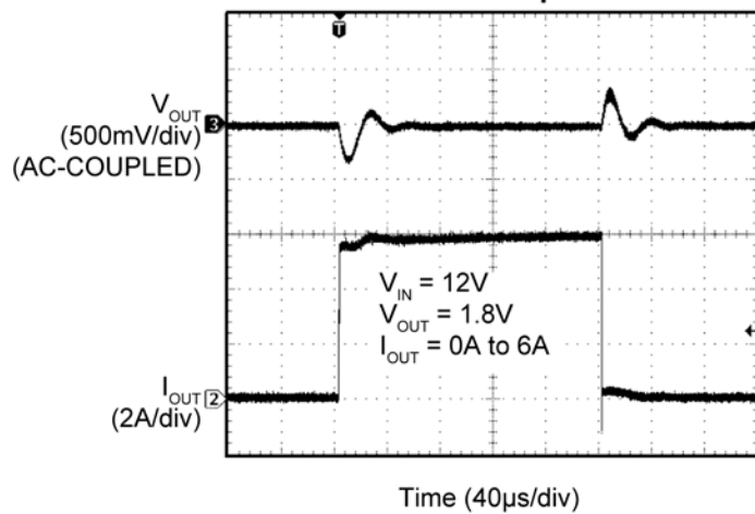
Transient Response
