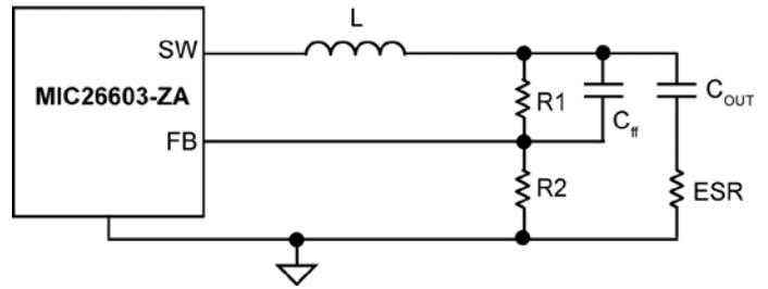
Figure 6. Inadequate Ripple at FB
