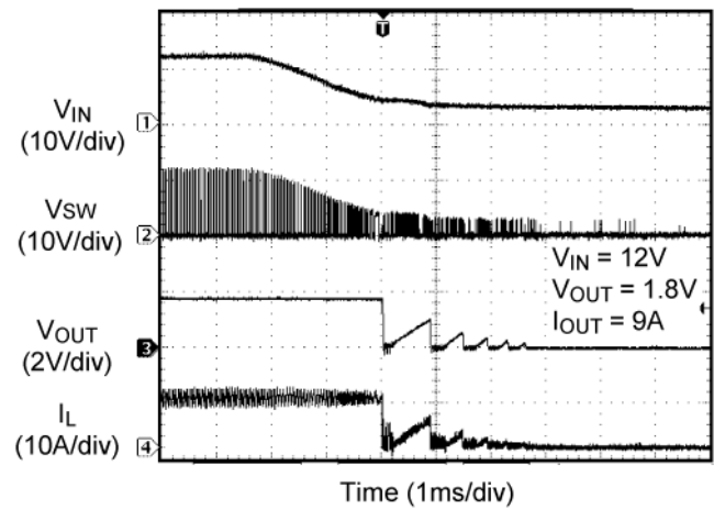
V IN Soft Turn-Off
