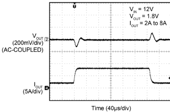
Transient Response
