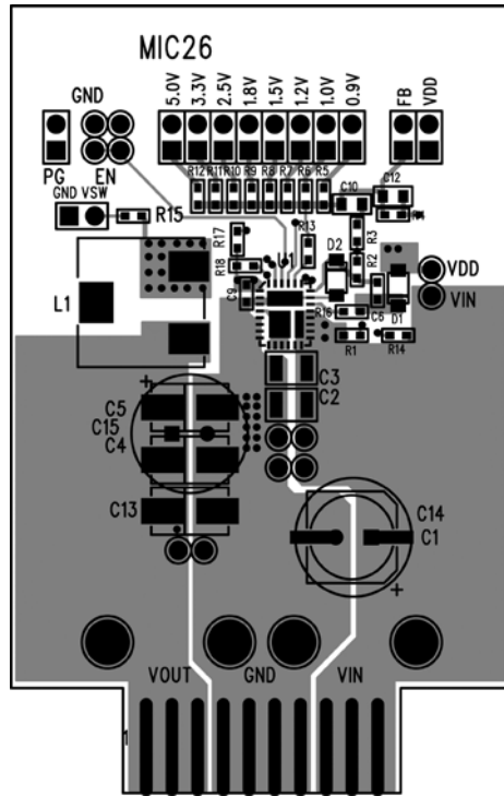
MIC26903-ZA Evaluation Board Top Layer
