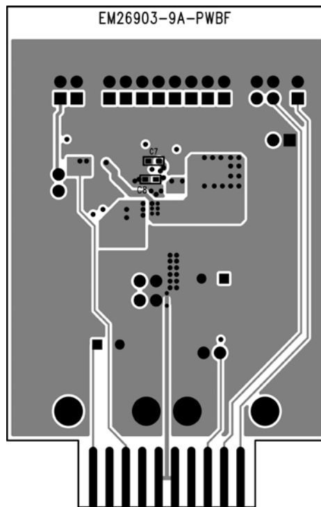
MIC26903-ZA Evaluation Board Bottom Layer
