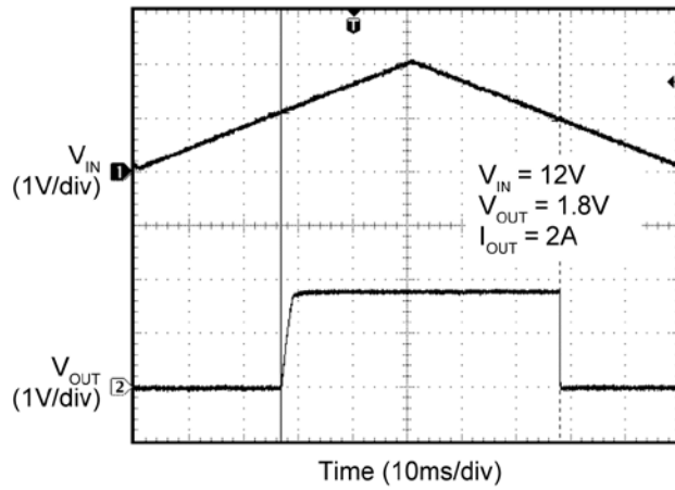
Enable Thresholds
