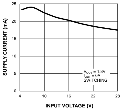
V_{IN} Operating Supply Current vs. Input Voltage
