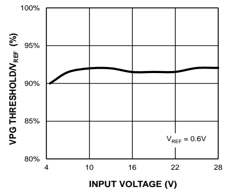
PG/V_{REF} Ratio vs. Input Voltage
