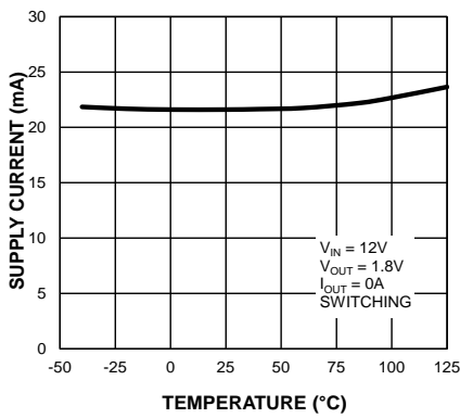
V IN Operating Supply Current vs. Temperature
