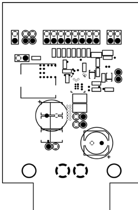
MIC26903-ZA Evaluation Board Mid-Layer 1 (Ground Plane)
