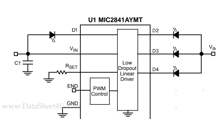
LCD Display Backlight with Four WLEDs
