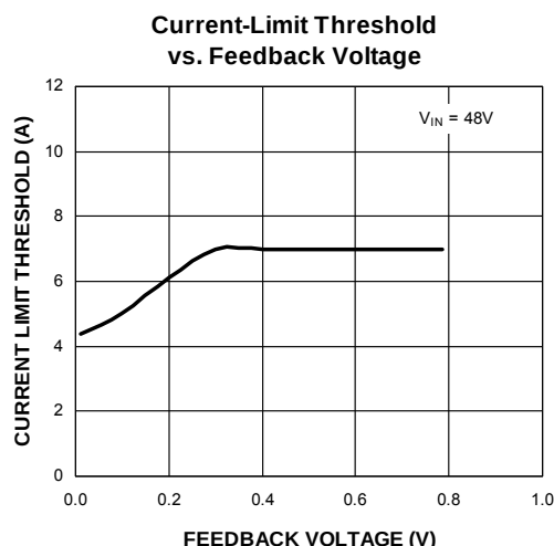
Figure 4. MIC28510 Current-Limit Foldback Characteristic
