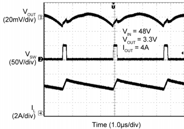
Switching Waveforms: I_{OUT} = 4A
