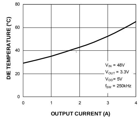
Die Temperature* ( V_{IN} = 48V ) vs. Output Current
