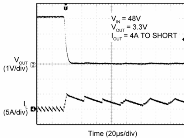
Short Circuit
