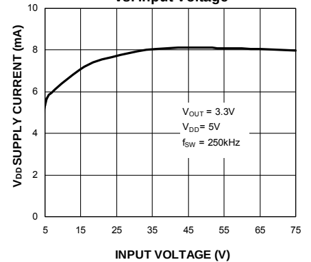
V_{DD} Operating Supply Current vs. Input Voltage
