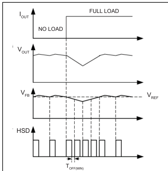
FIGURE 4-3: MIC28511 Load Transient Response.
