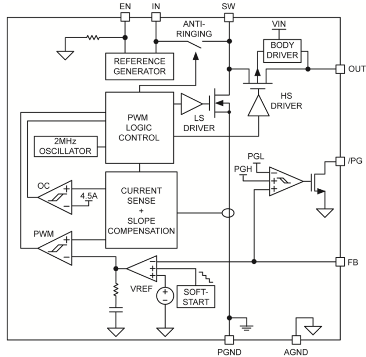
Simplified Adjustable Output Functional Diagram
