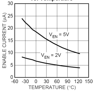
D2632 Enable Current vs. Temperature
