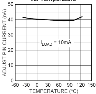
D2632 Adjust Pin Current vs. Temperature
