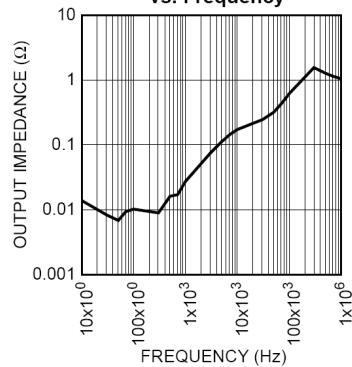
D2632 Output Impedance vs. Frequency
