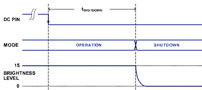
Figure 3. Shutdown Timing
