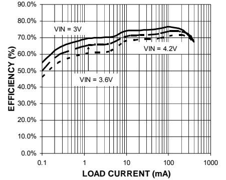
Efficiency vs. Load (V OUT = 1.5V)
