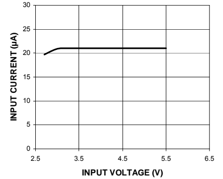
Quiescent Current vs. Input Voltage (Not Switching)
