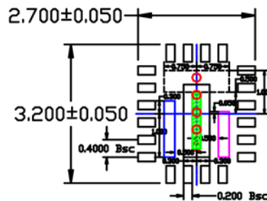
BOTTOM VIEW NOTE 1,2,3
