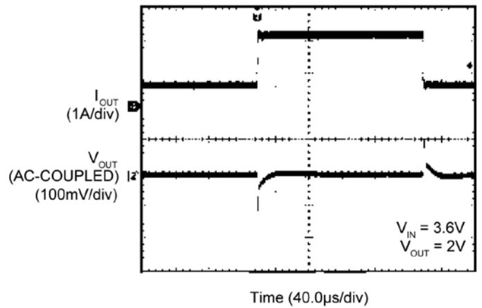
Load Transient (250mA – 2A)
