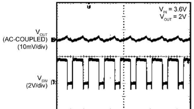
Switching Waveform Continuous Mode (2A)
