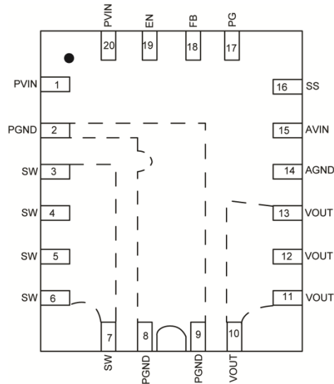
2.5mm x 3mm QFN (GK) (Top View)
