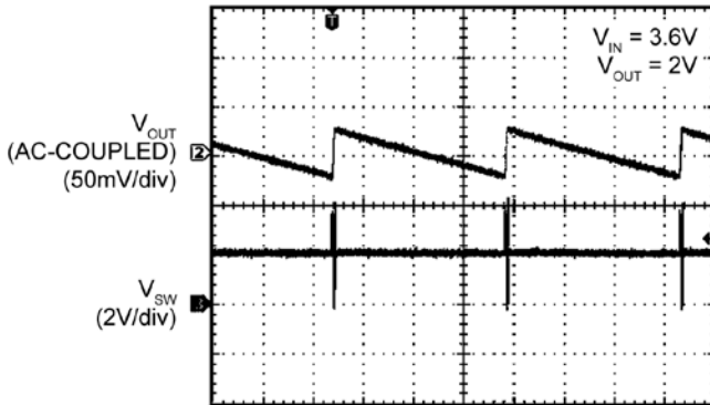
Switching Waveform Discontinuous Mode (10mA)
