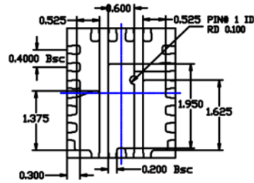
BOTTOM VIEW NOTE 1,2,3
