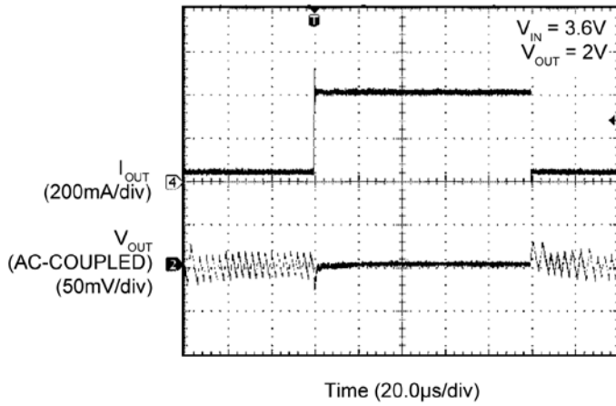
Load Transient (50mA – 400mA)
