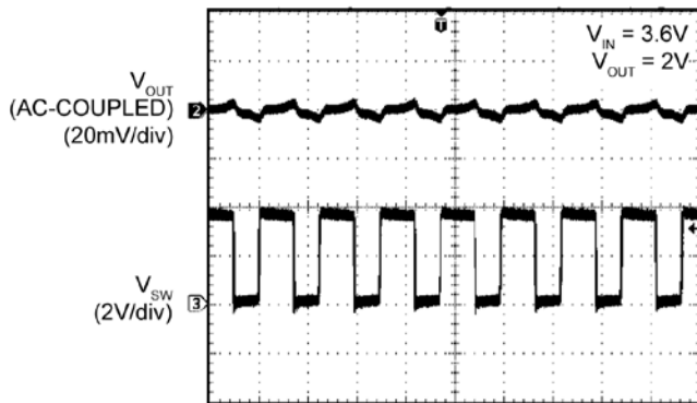
Switching Waveform Continuous Mode (200mA)
