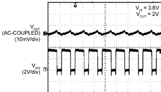
Switching Waveform Continuous Mode (1.5A)
