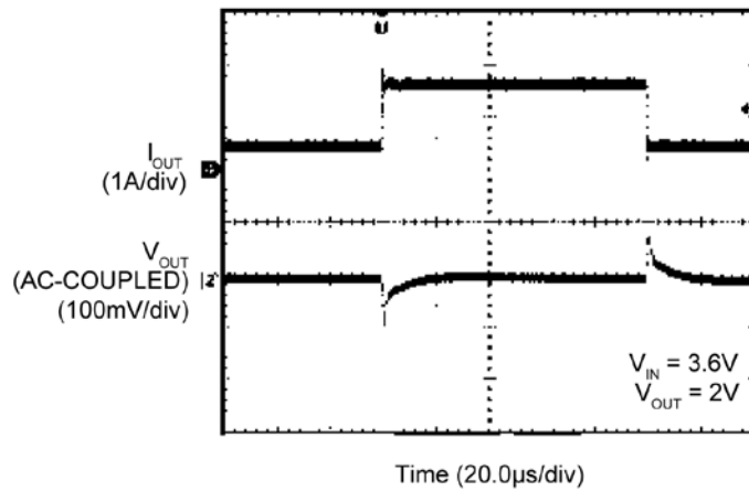
Load Transient (250mA – 1.5A)
