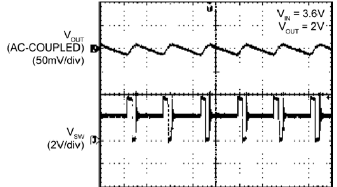
Switching Waveform Discontinuous Mode (50mA)
