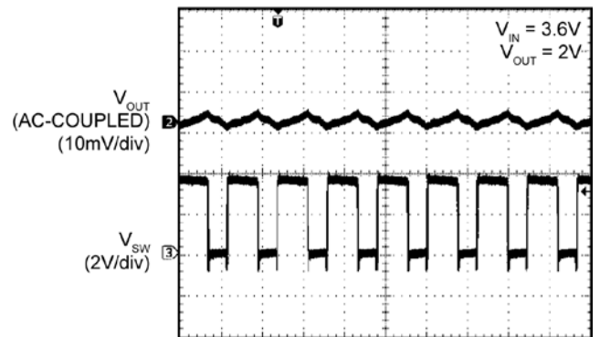
Switching Waveform Continuous Mode (800mA)
