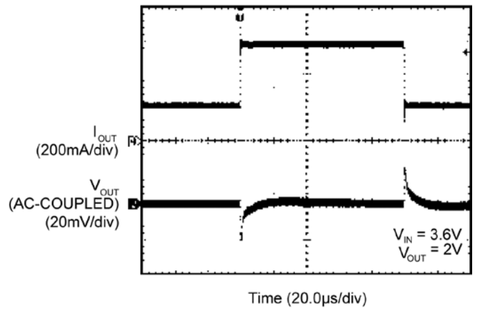
Load Transient (200mA – 600mA)
