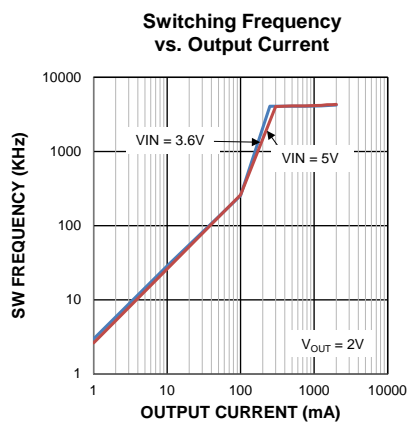
Figure 3. SW Frequency vs. Output
