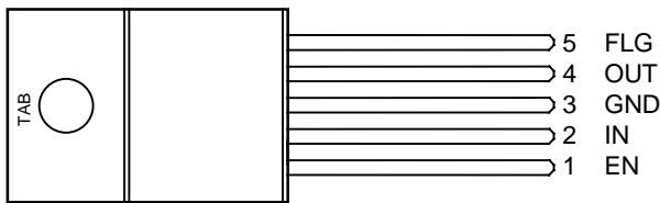
MIC39301-x.xBT TO-220-5 (T)
