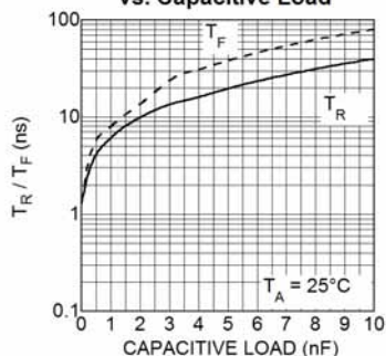
Rise and Fall Time (5V) vs. Capacitive Load
