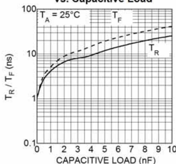
Rise and Fall Time (12V) vs. Capacitive Load
