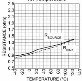
Output Impedance (12V) vs. Temperature
