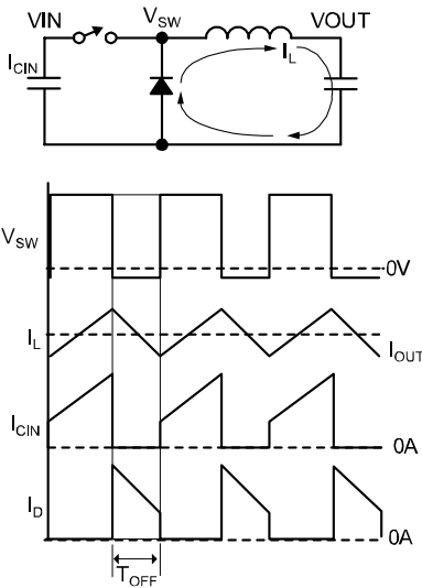
Figure 4. Off-Time
