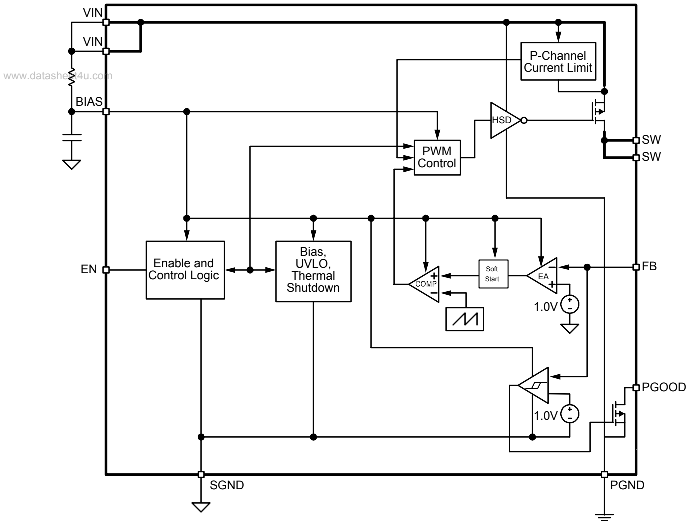
MIC4722 Block Diagram
