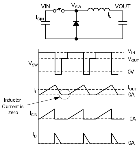
Figure 5. Discontinuous Operation
