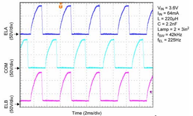
Figure 4. EL Panel Waveform – 2 × 3 in 2
