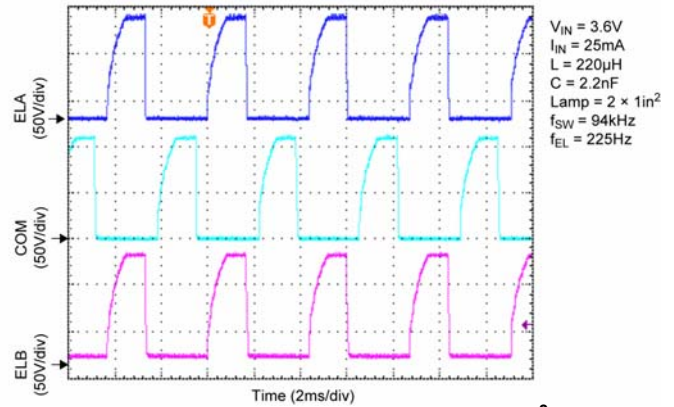
Figure 2. EL Panel Waveform – 2 × 1 in 2
