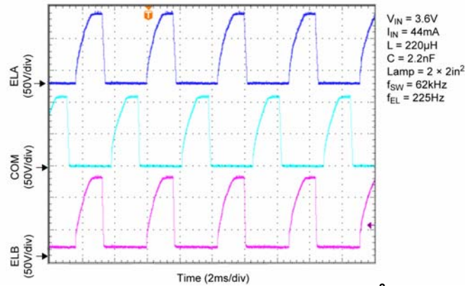
Figure 3. EL Panel Waveform – 2 × 2 in 2
