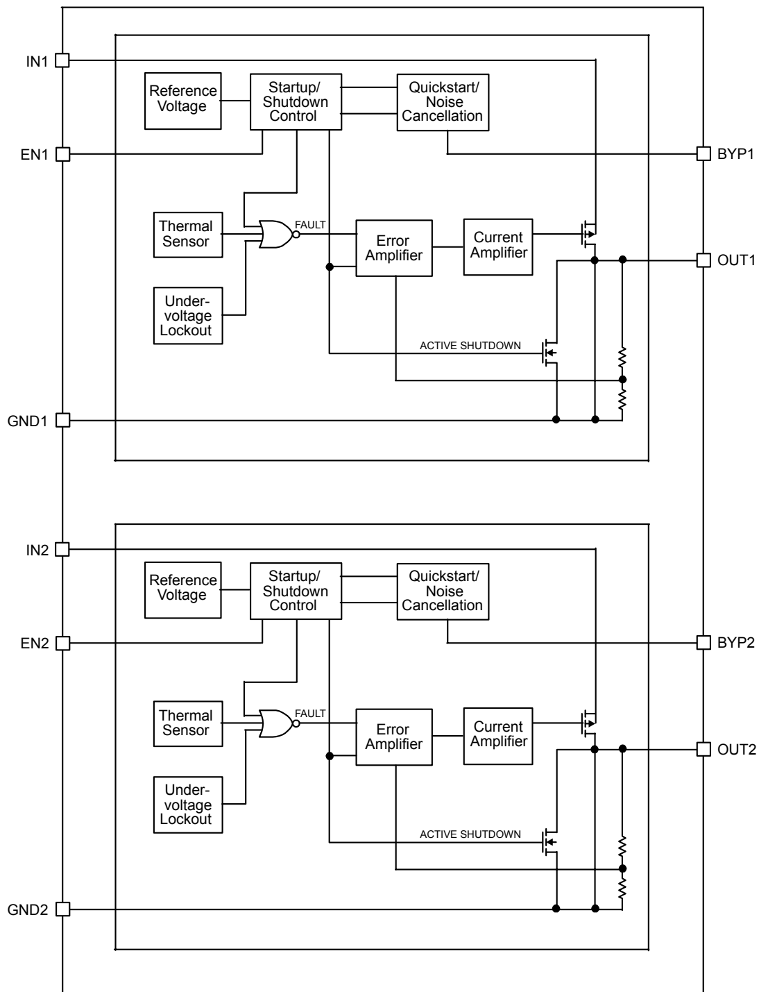
MIC5264 Diagram
