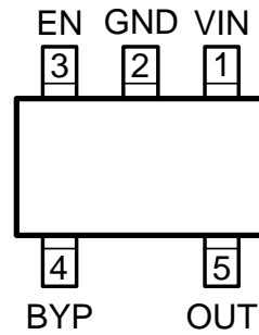
Lead-Free Thin SOT-23-5 (YD5)
