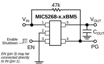
1.2V Regulator with Power Good
