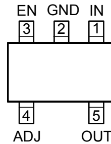
5-Pin Thin SOT23 (D5) Adjustable (Top View)
