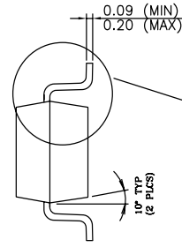
END VIEW
