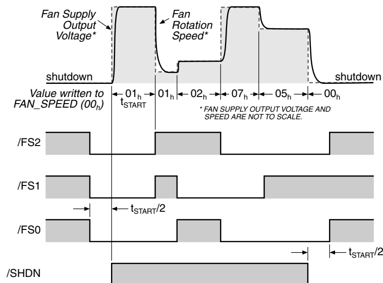
Figure 2. Typical MIC74 Fan-Mode Timing and System Behavior
