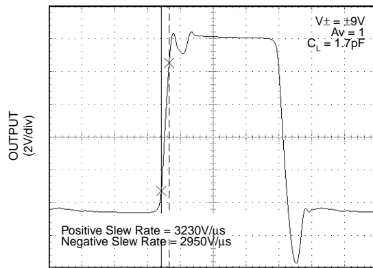
TIME (25ns/div)
