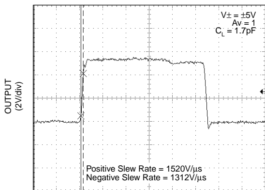
TIME (25ns/div)
