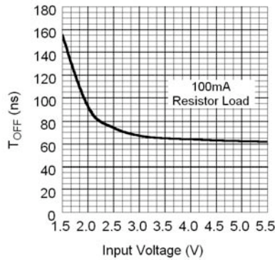
T OFF Delay vs. Input Voltage
