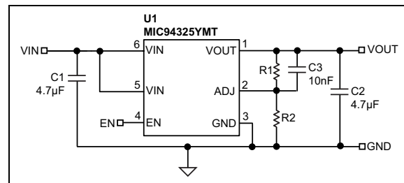
FIGURE 4-1: Adjustable Output Voltage.
