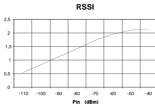
Figure 9. RSSI Voltage
