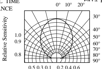
FIG.5 SENSITIVITY DIAGRAM
