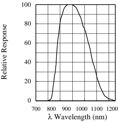
FIG.5 RELATIVE SPECTRAL SENSITIVITY VS. WAVELENGTH
