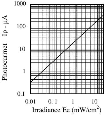
FIG.6 PHOTOCURRENT VS. IRRADIANCE = 950 nm
